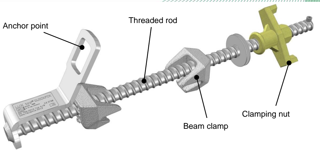
Fig. 1: Anchor device, type: LUX-top® QUICKFIX
