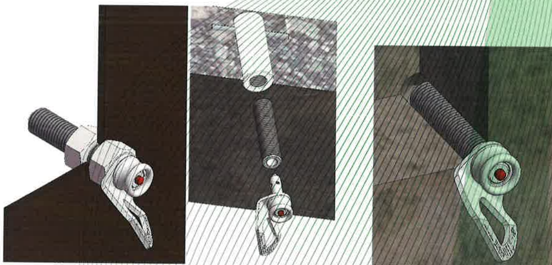
Fig. 1-3: Anchor device, type LUX-top® KLICK SZP
