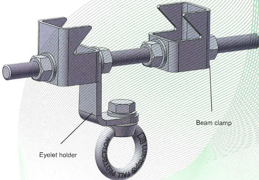
Fig. 1: Anchor device, type: LUX-top® QUICKFIX II
